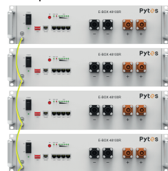
Multiple Batteries
