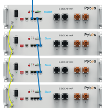
Multiple Batteries
