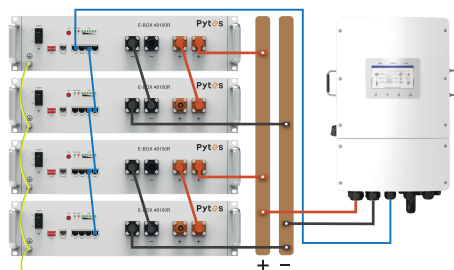
Multiple Batteries
